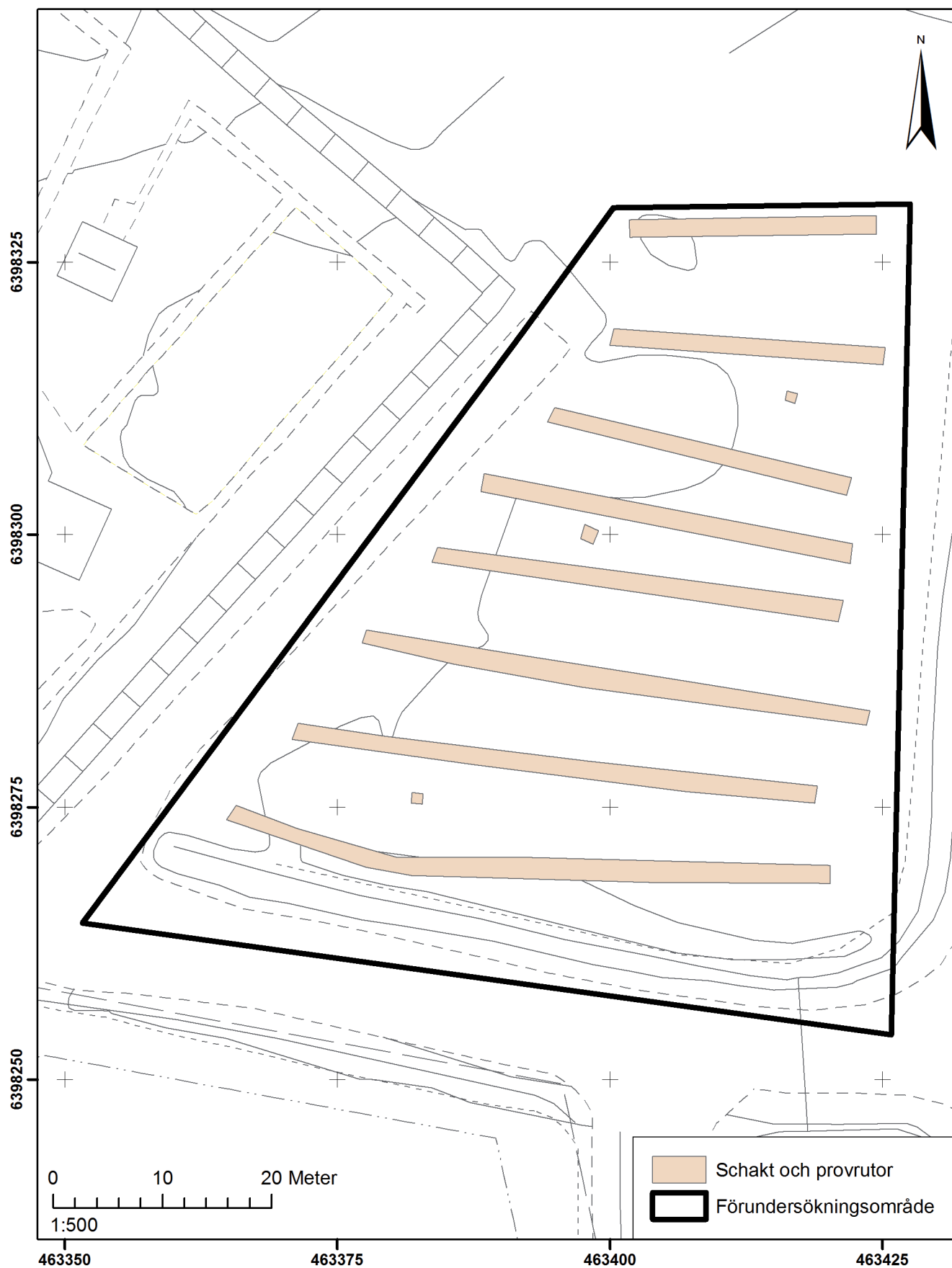
Schaktplan. Skala 1:500.
