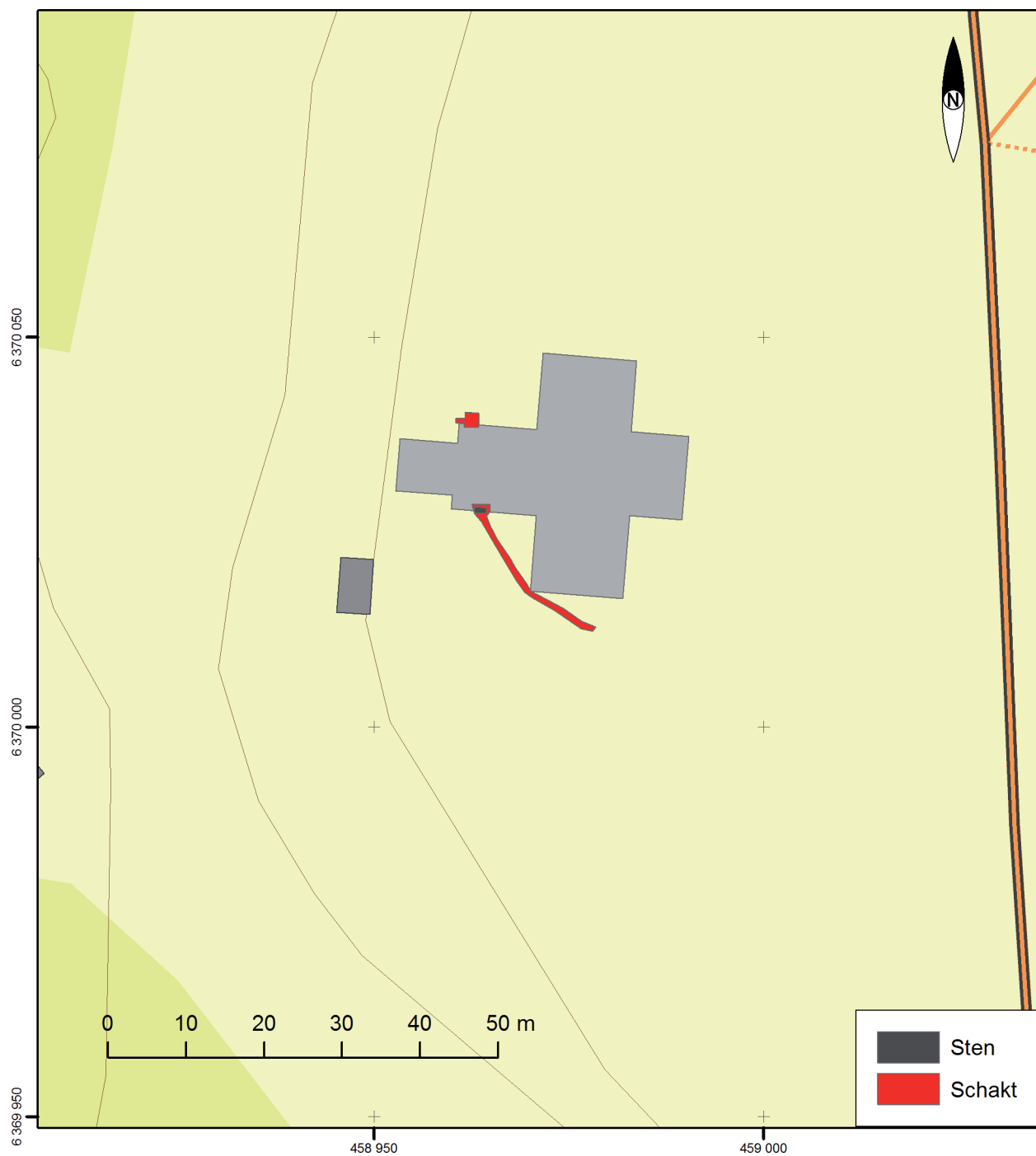
Figur 2. Schaktplan. Skala 1:800.
